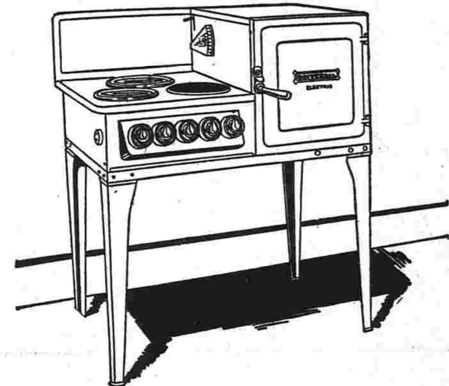
No. 2593 White and Gray Porcelain Enamel Finish with Nickel Plated Trim. Oven temperature control. Pilot light, oven temperature indicator. Open and closed units interchangeable.
